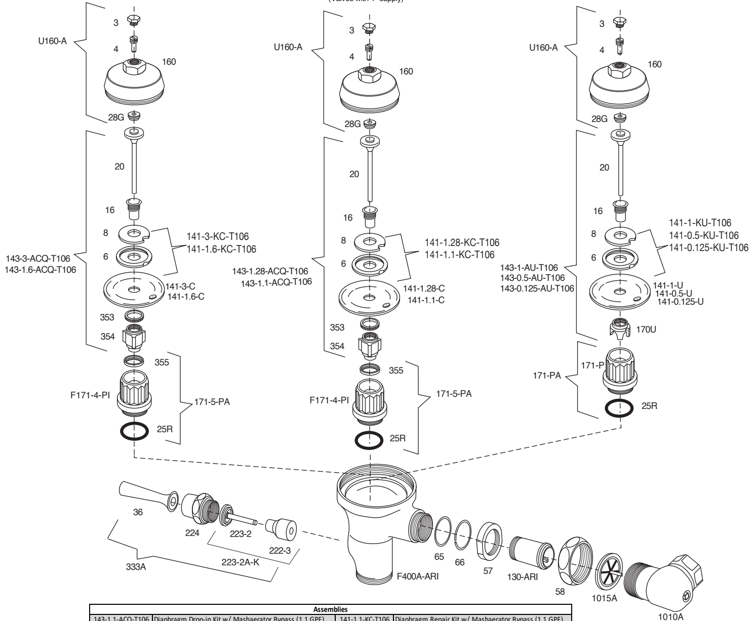
UP451-1 / U451-0.5 / UP451-0.125 (Valves with 3/4" supply)
